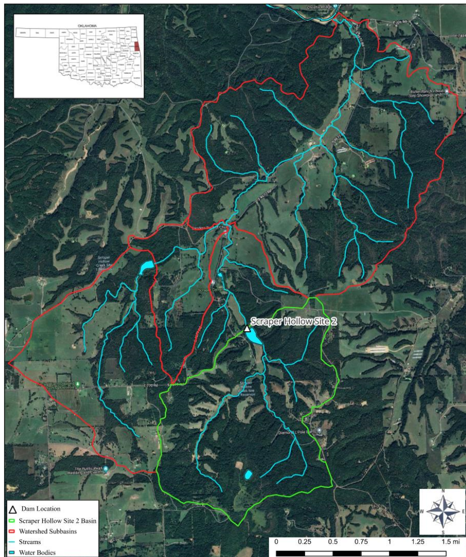
Figure 1: Location of Scraper Hollow FWRS No. 2 in Adair County, Oklahoma
